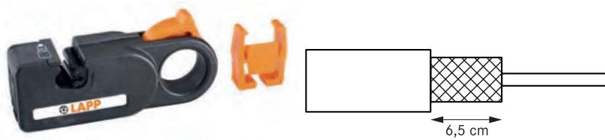
FC STRIP stripping tool
